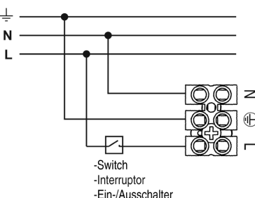
NO DIMMING Diagram W
